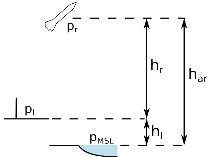
Figure A.2. Visualization of pressure measurements and height calculations. p_{MSL} is pressure at mean sea level (101.325 kPa), p_l is pressure at measured at launchpad (reference pressure), from which h_l , absolute altitude of launchpad is calculated. p_r is pressure measured by Arecorder during the flight; from this pressure absolute altitude of rocket ( h_{ar} ) is calculated.
