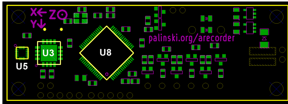
Figure 6.3. Location of important components on bottom side of Arecorder's PCB board.
