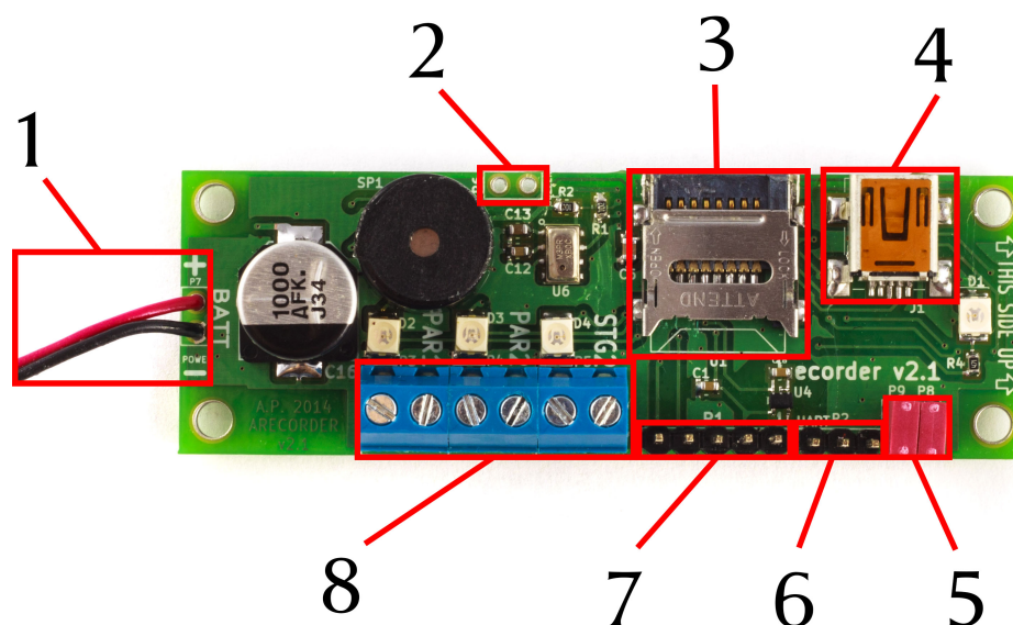
Figure 2.1. Arecorder's connectors.
